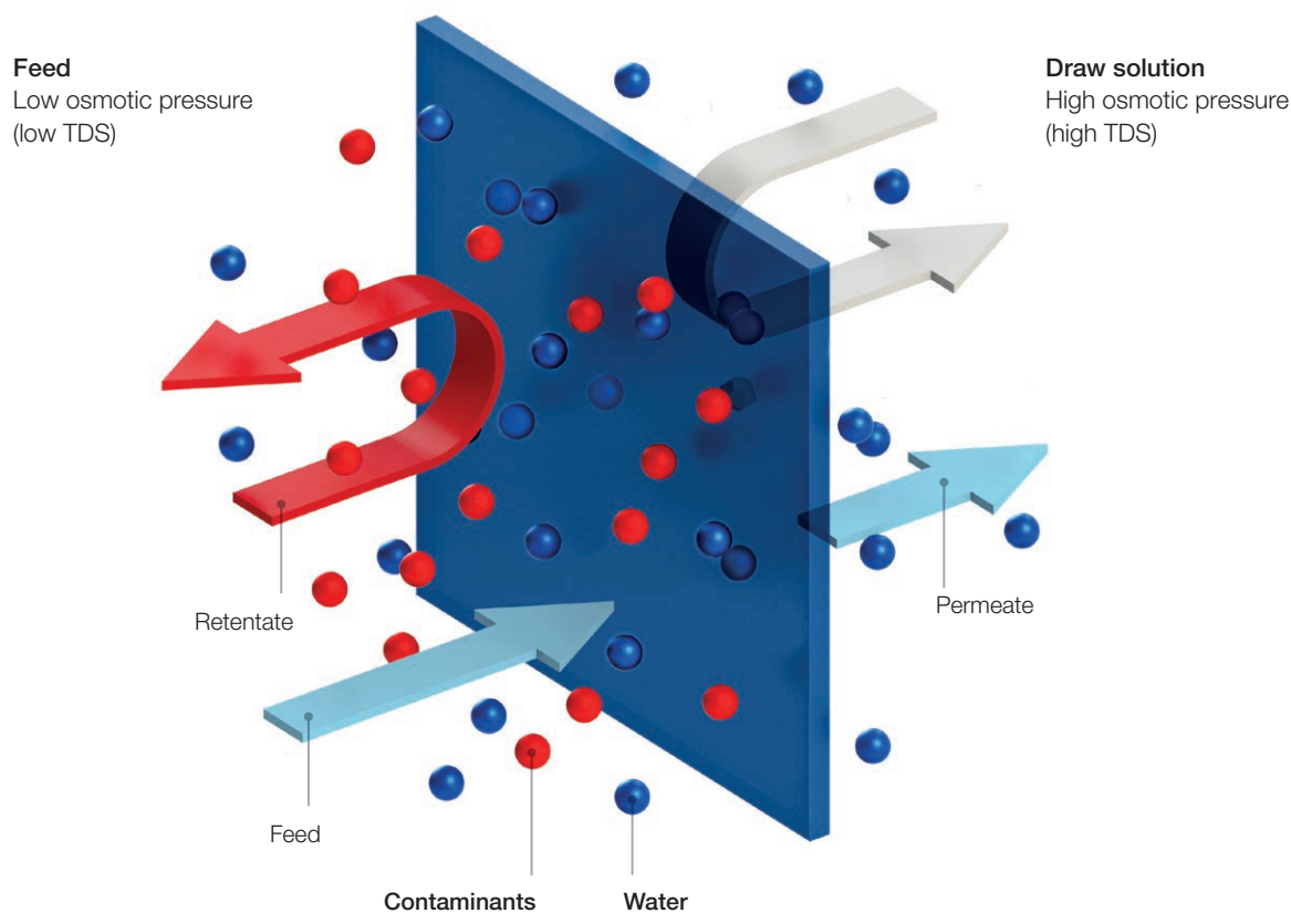
Figure 1: Principle of forward osmosis
