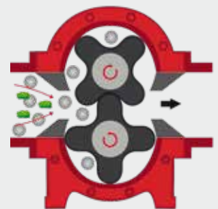
Rotary lobe pump with InjectionSystem
